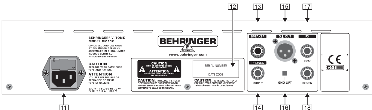
Fig. 2.2: Rear panel connectors
